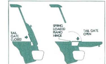
A-634 Cover Plate for Tailgate Aperture, operates automatically—no gaps for cot wheels to drop into.
