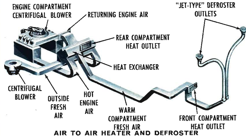
AIR TO AIR HEATER AND DEFROSTER
