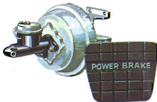
POWER BRAKES A low pedal type power brake that brings the truck to a smooth, positive stop. Available for all 1/2 to 1 ton trucks.
