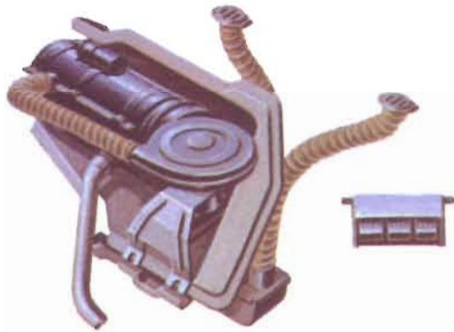
GASOLINE HEATER AND DEFROSTER FOR ALL SERIES 95 TRUCKS
