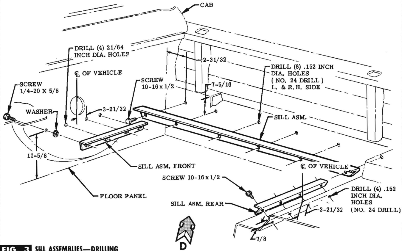
FIG. 3 SILL ASSEMBLIES—DRILLING
